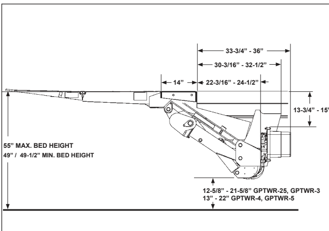
GPTWR Lift Dimensions and Mounting Requirements
